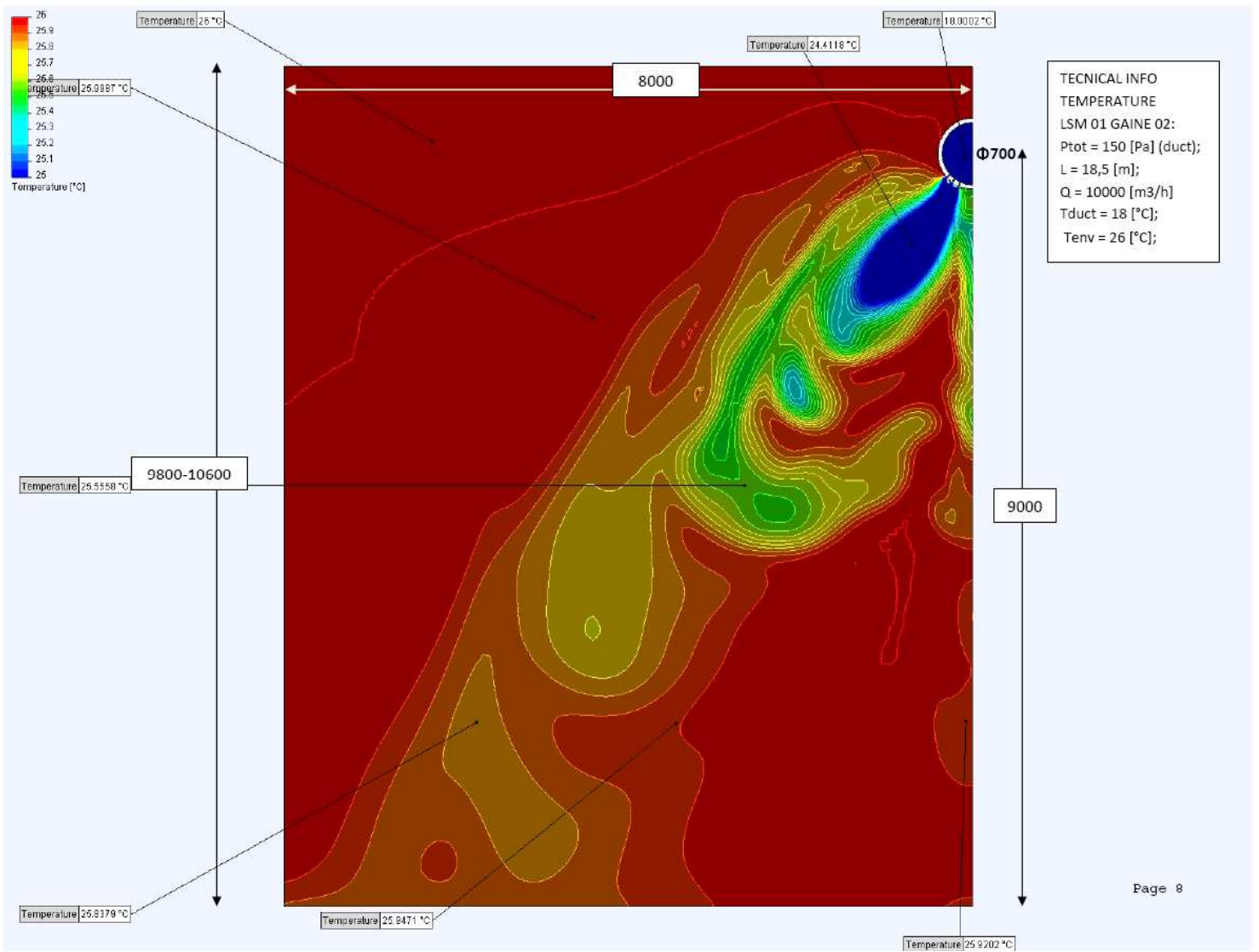
Example of a CFD simulation with velocity values at each point.
