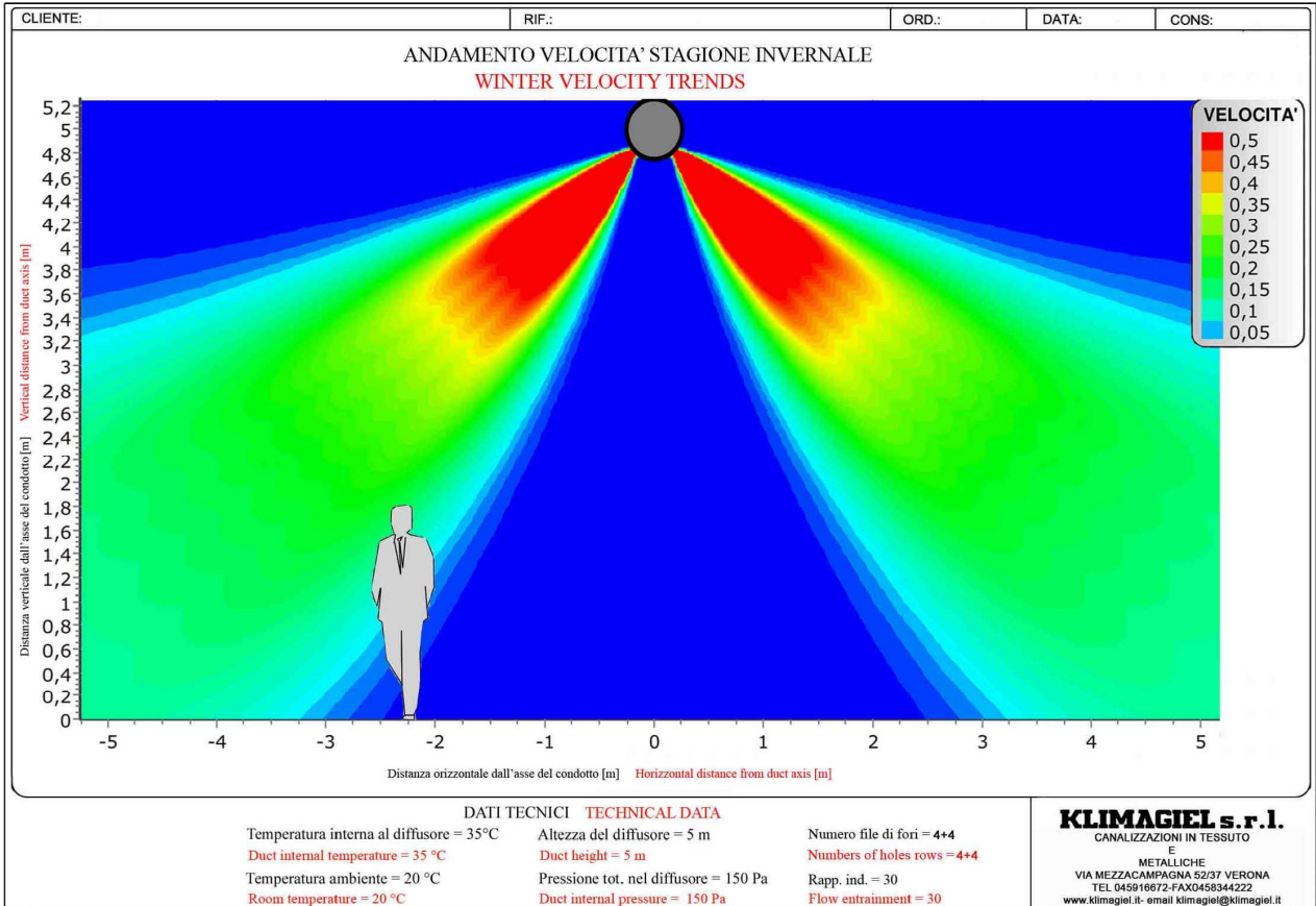
Air throw pattern from this JET-IN diffuser in heating application (winter).
