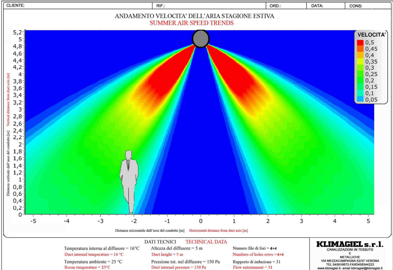
Air throw pattern from the same JET-IN diffuser in cooling application (summer).
